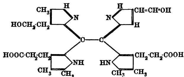
Haematoporphyrin, C_{38}H_{38}O_6N_4 .
